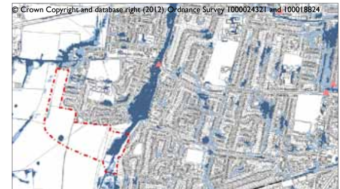
Figure 12e- Surface Water Flooding
