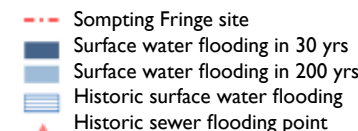
Figure 12e- Surface Water Flooding
