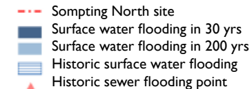
Figure 11e - Surface Water Flooding
