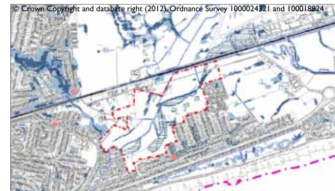
Figure 14e - Surface Water Flooding
