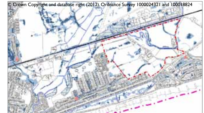
Figure 15e - Surface Water Flooding
